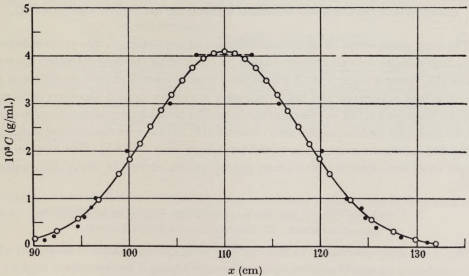
FIGURE 7. Initially asymmetrical distribution which has become symmetrical owing to dispersion. \circ , C = 0.0041 \exp \{-(110-x)^2/121\} ; \bullet , experiment; time = 11 min.
